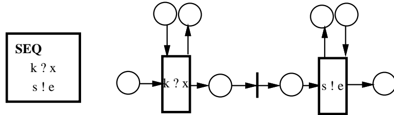
Figura 5.6: Sequence
