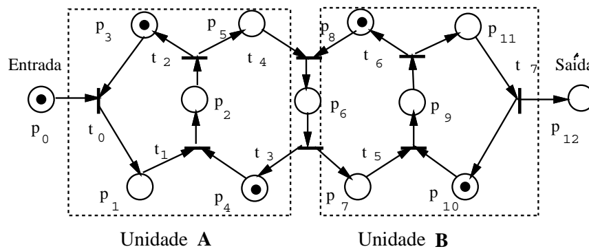
Figura 2.15: Pipeline
