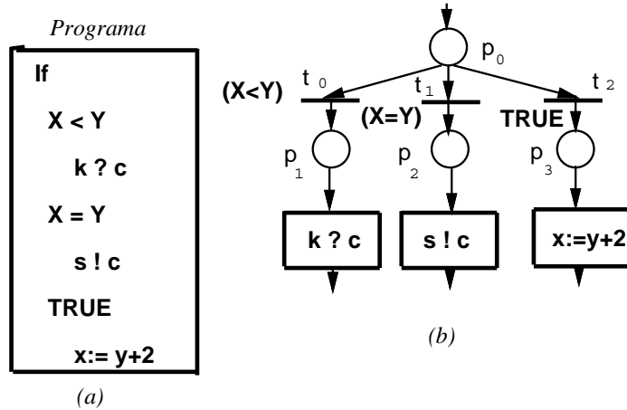
Figura 5.7: Conditional
